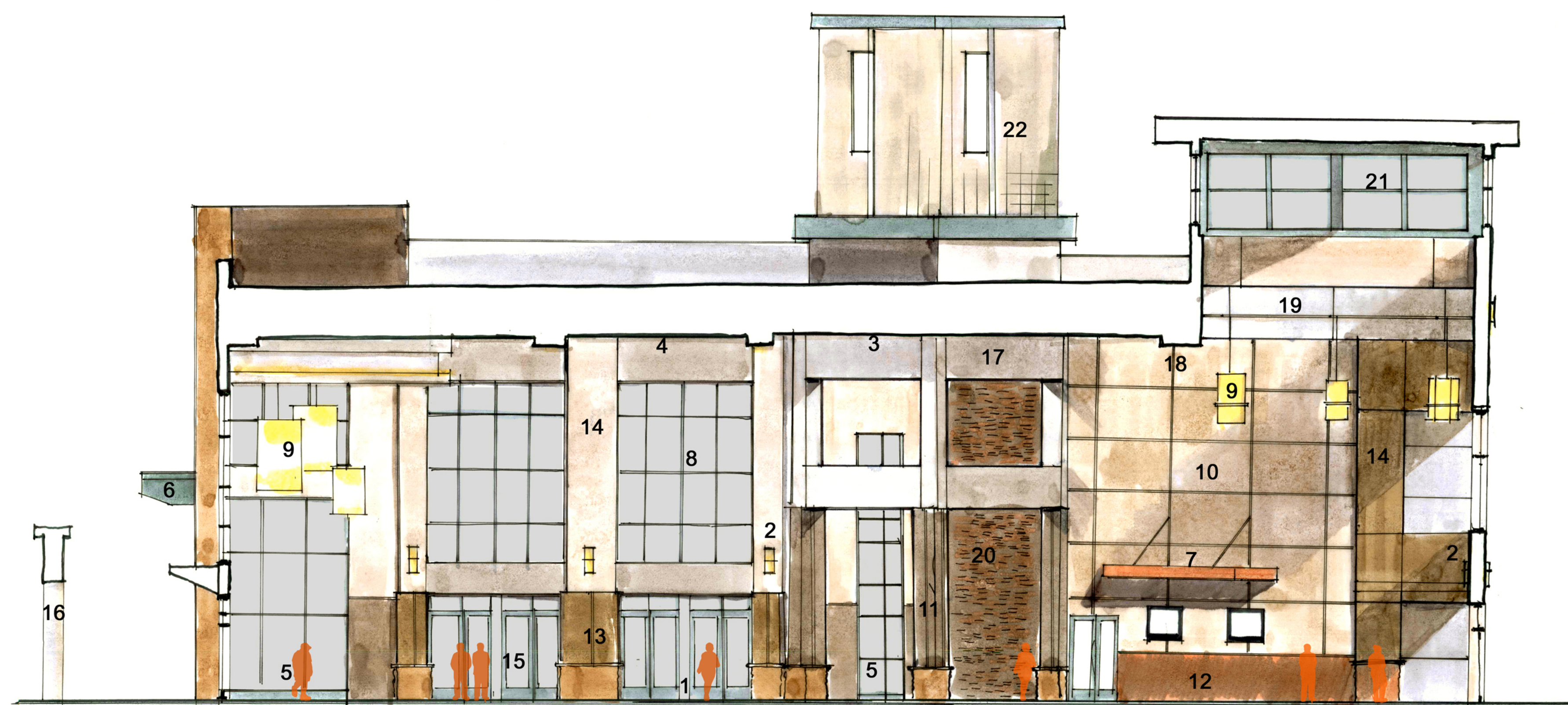
EAST FACING LOBBY INTERIOR ELEVATION
